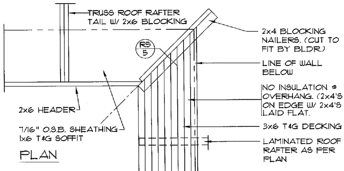
TRUSS ROOF / 3X6 DECKING VALLEY DETAIL WITH 5" RIGID INSULATION
